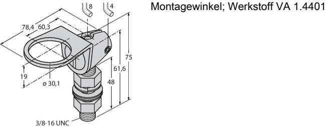
SMB30FA 3074005
