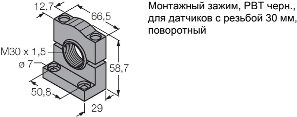
SMB30SC 3052521
