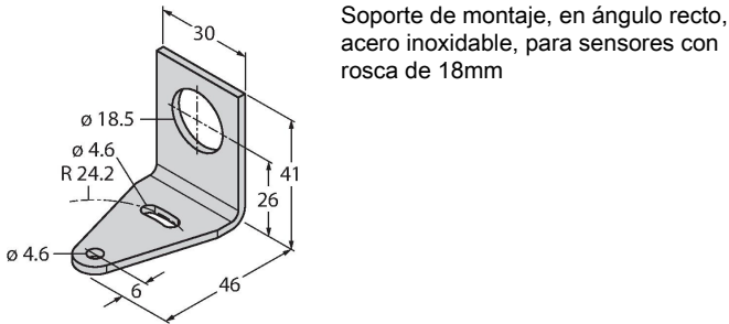
SMBAMS18P 3073134
