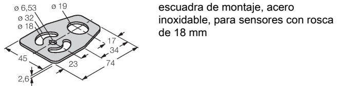
SMBAMS18P 3073134
