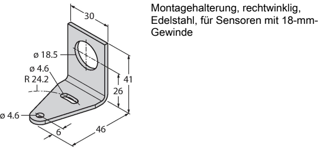
SMB3018SC 3053952
