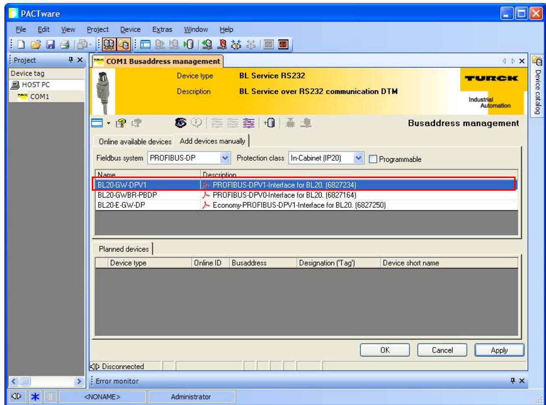
Figure 4-4: Selecting the gateway
