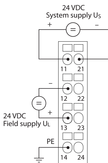
Figure 2-2: Pin assignment BL20-BR- 24VDC-RED
