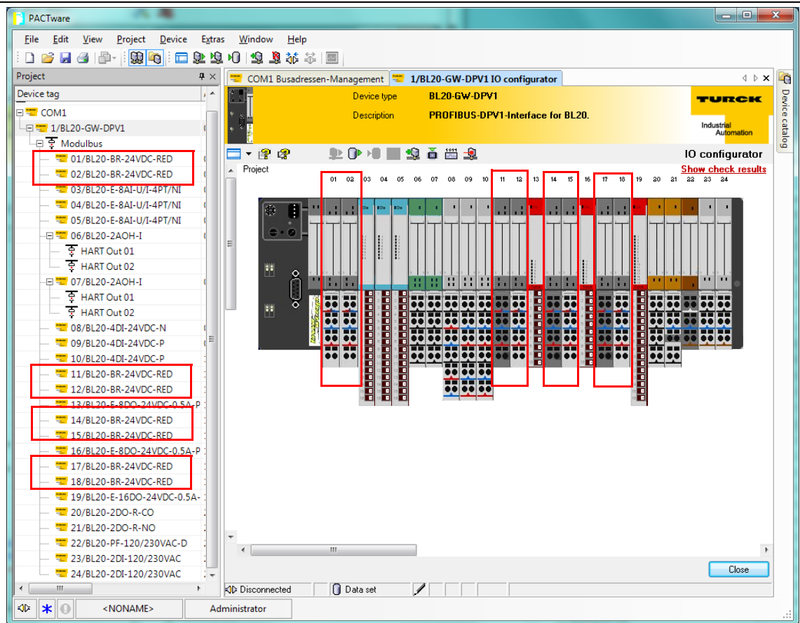
Figure 4-6: I/O-configuration with redundant Bus Refreshing mod- ules
