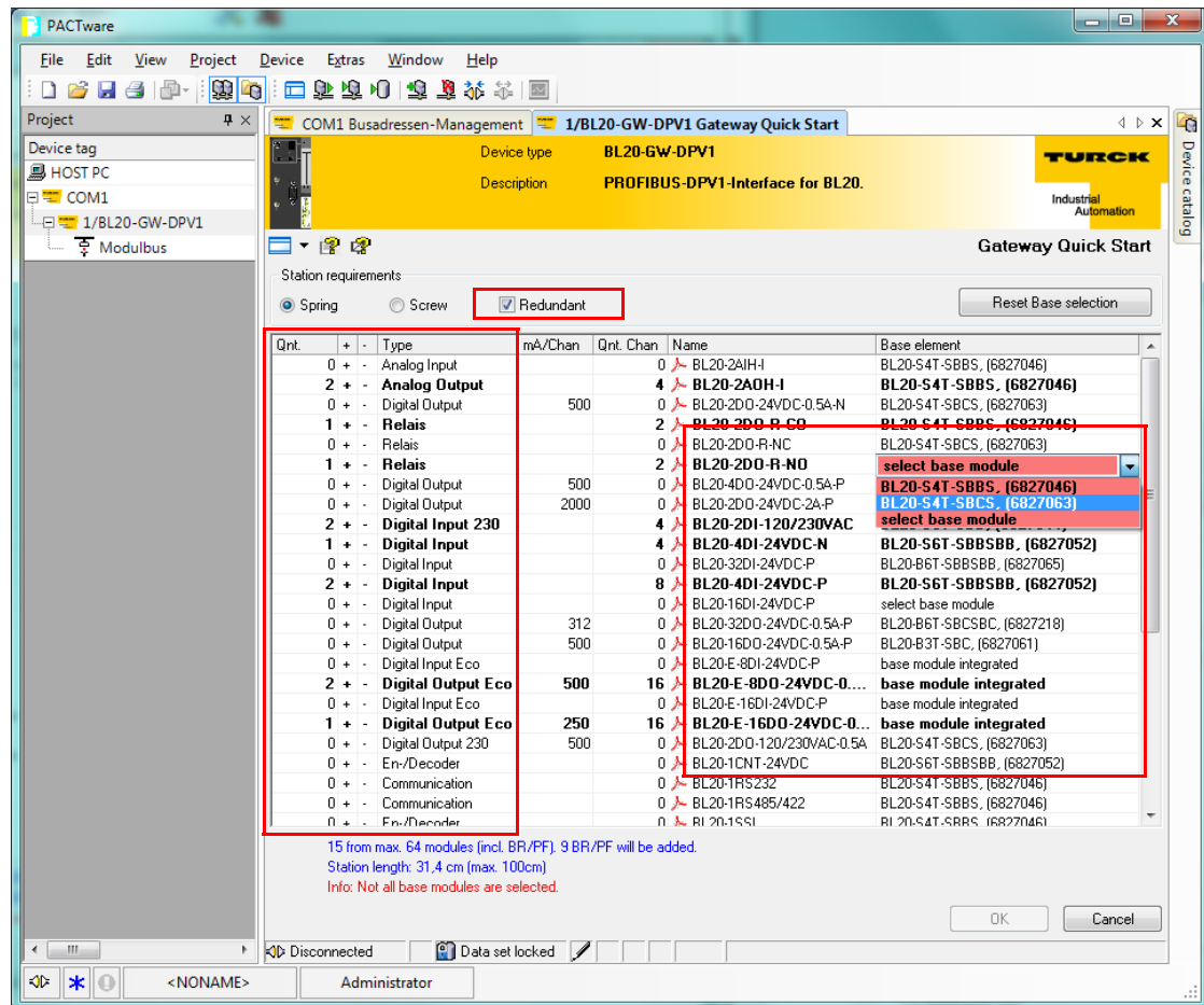
Figure 4-5: Activating the redundancy and defining the number and type of required I/O- channels
