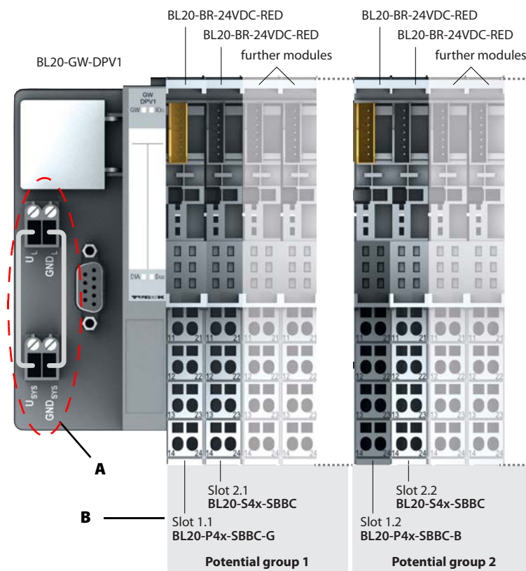
Figure 3-1: Station assembly with BL20-GW-DPV1 and redundant power supply
