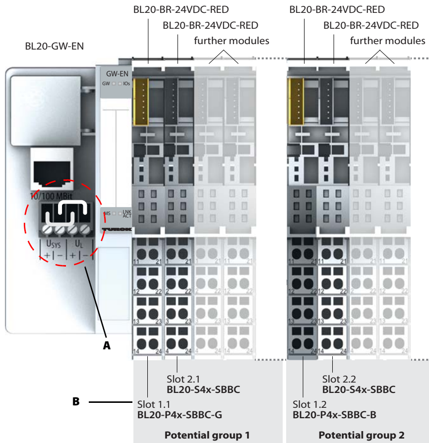
Figure 3-2: Station assembly with BL20-GW-EN and redundant power supply
