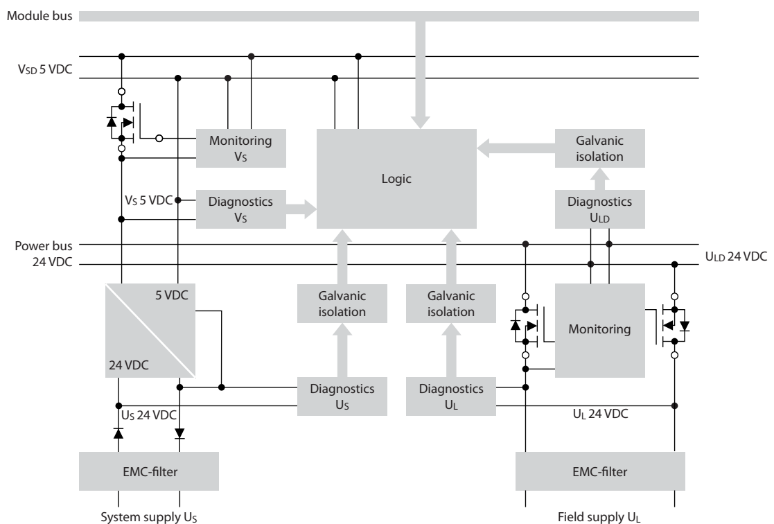
Figure 2-1: Block diagram of one single BL20-BR- 24VDC-RED
