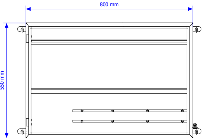
MOUNTING VIEW
