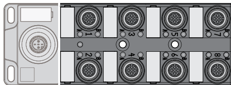
Fig. 4: M12 connector for connecting digital sensors (C1...C8)
