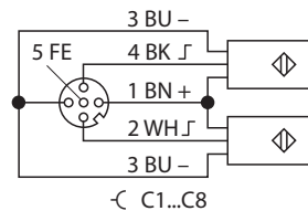
Fig. 5: Pin assignment TBIL-M1-16DIP (C1...C8)
