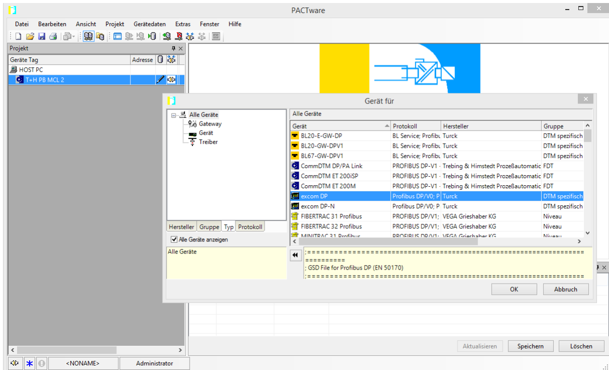
Abb. 3: Adding an excom® station
